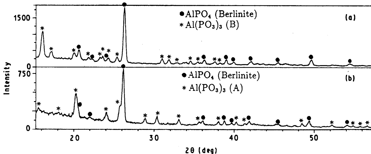
Figure 3 XRD patterns of the phosphate A01 after heat treatments at (a) 500 and (b) 800 °C.
