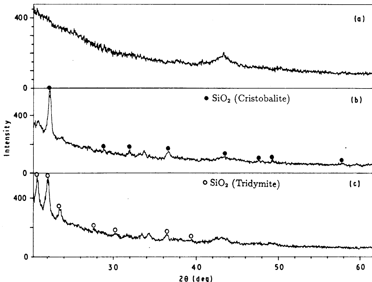
Figure 11 XRD patterns of the water glass after heat treatments at (a) 200, (b) 800 and (c) 1100 °C (in air).
